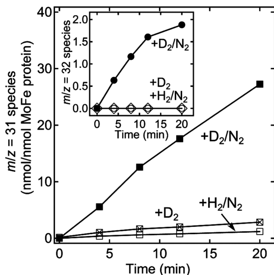
Figure 17. Time-dependent formation of ^{13}\text{C}_2\text{H}_3\text{D} and ^{13}\text{C}_2\text{H}_2\text{D}_2 , catalyzed by nitrogenase reduction of ^{13}\text{C}_2\text{H}_2 . ^{13}\text{C}_2\text{H}_3\text{D} determined by GC/MS monitoring of m/z = 31 for a reaction mixture containing ^{13}\text{C}_2\text{H}_2 and including \text{D}_2 and \text{N}_2 (■), just \text{D}_2 (x inside □), or \text{H}_2 and \text{N}_2 (□). Inset: ^{13}\text{C}_2\text{H}_2\text{D}_2 , m/z = 32 , formation starting with ^{13}\text{C}_2\text{H}_2/\text{D}_2/\text{N}_2 (●), just \text{D}_2 (◇), or \text{H}_2/\text{N}_2 (○). Partial pressures of 0.02 atm ^{13}\text{C}_2\text{H}_2 , 0.25 atm \text{N}_2 , and 0.7 atm \text{H}_2/\text{D}_2 , where present. The molar ratio of Fe protein to MoFe protein was 2:1. All assays incubated at 30 °C. Adapted with permission from ref 157. Copyright 2013 National Academy of Sciences.
