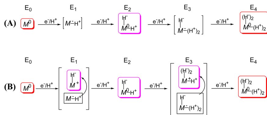
Figure 6. Formulations of E_1 – E_4 derived from consideration of E_4 as containing two bound hydrides and two protons. (A) Assuming reduction of the core in n = 1, 3 states. (B) Alternative formulation of E_1 – E_4 under the assumption of hydride formation at every stage, in which case the core is formally oxidized for E_n , n = 1, 3 . Symbols: M represents FeMo-co core; superscripts are charge difference between core and that of resting-state (commonly denoted M^N ); the number of bound protons/hydrides are indicated. Adapted with permission from ref 156. Copyright 2013 American Chemical Society.
