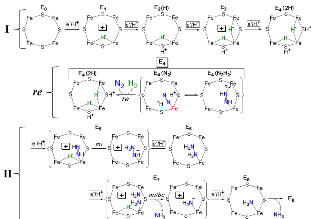
Figure 19. Proposed mechanism displaying structures of all intermediates in nitrogen fixation, inspired by the assumption of primacy of hydride chemistry associated with the Fe 2,3,6,7 face of FeMo-co, and containing a formal description of the transformations that convert each stage to the subsequent one. In I the mechanism tentatively adopts and visualizes the view of E n states n = 1-4 presented in Figure 6B; in II it visualizes bridging hydrides by analogy, without evidence for or against terminal hydrides for n = 5-7 . Likewise, the structure of the N 2 H 2 species as end-on bound diazene is suggestive, not definitive, etc. I and II are connected by the re mechanism, Figure 13, lower. Formal charges are included as useful to help guide the reader.
